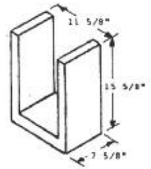
HI LINTEL
