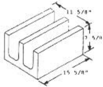
BOND BEAM
